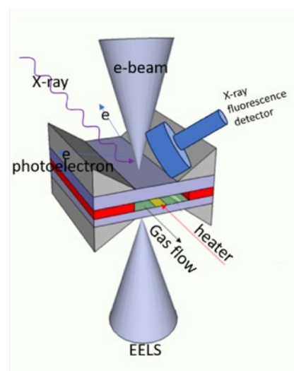
Figure 2-7: Nanoreactor for gas-solid reaction studies. It is compatible with TEM, X-ray microscopy, and XPS and also offers electron energy loss spectroscopy.
